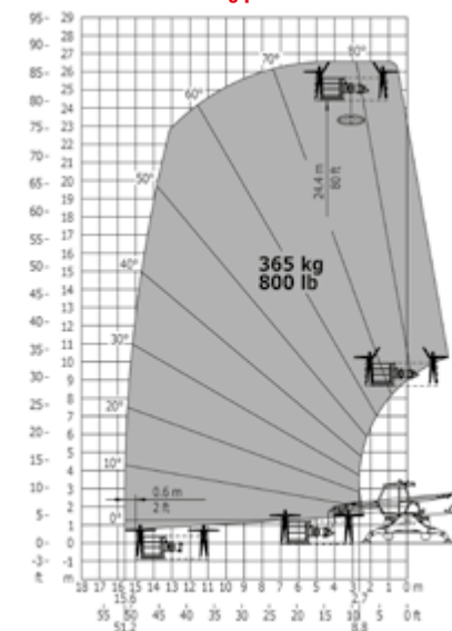
Rotation on lowered stabilisers with 365 kg platform
