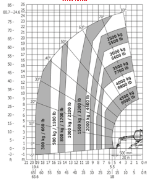
Rotation on lowered stabilisers with forks
