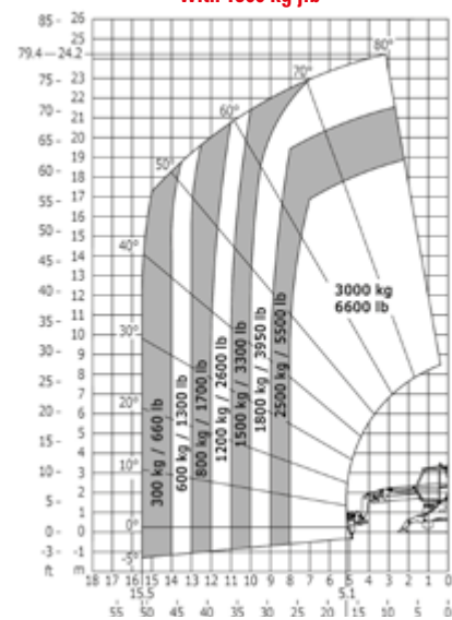
Rotation on lowered stabilisers with 1500 kg jib
